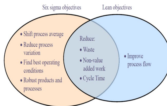
Figure 1. Improvement objectives (Source: Snee, 2010)
