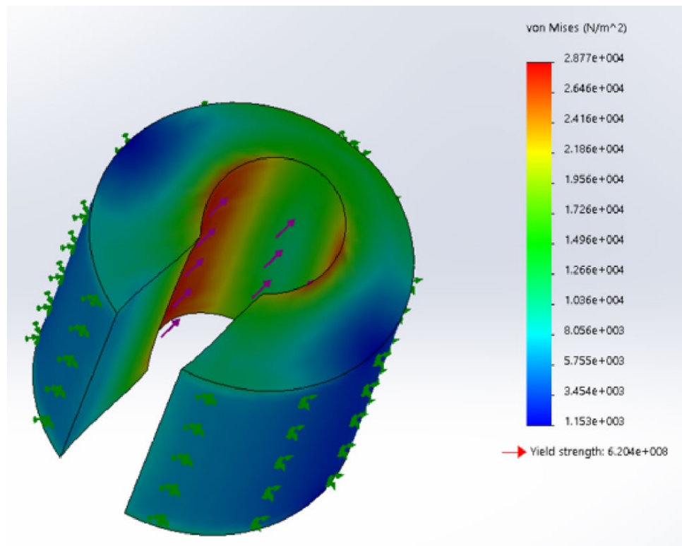
Figure 5. Finite Element Analysis (von Mises stress) of Tuned Mass Damper handle
