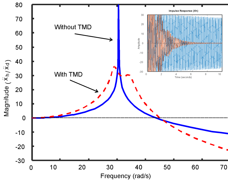
Figure 8. Frequency response function ( \ddot{x}_h/\ddot{x}_d ) and time response
