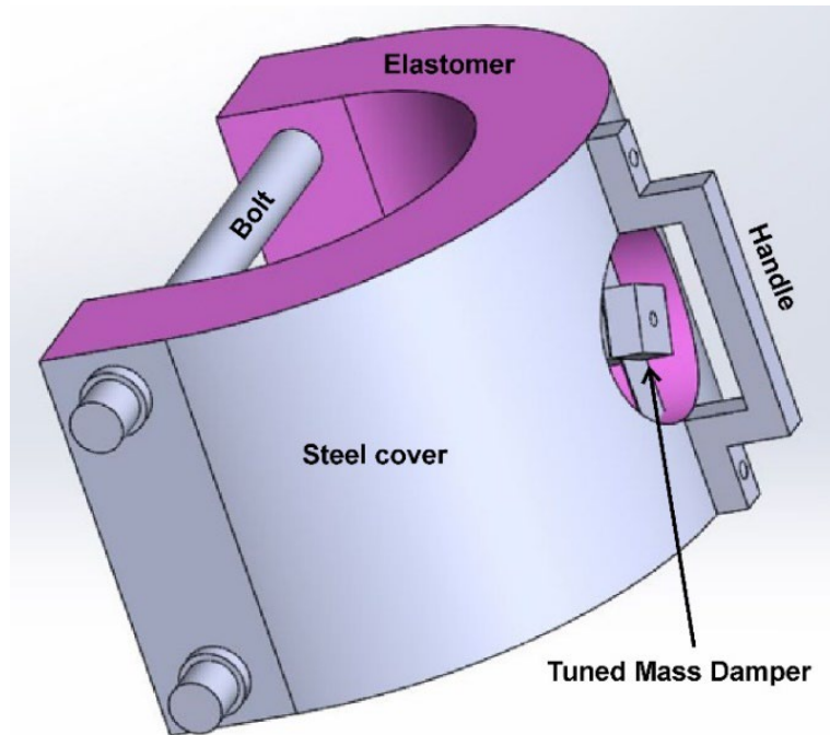
Figure 4. CAD design of Tuned Mass Damper handle
