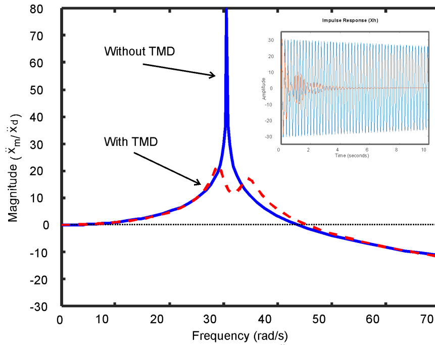
Figure 7. Frequency response function ( \ddot{x}_m/\ddot{x}_d ) and time response
