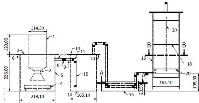
Figure 6 Prototype engineering drawing
