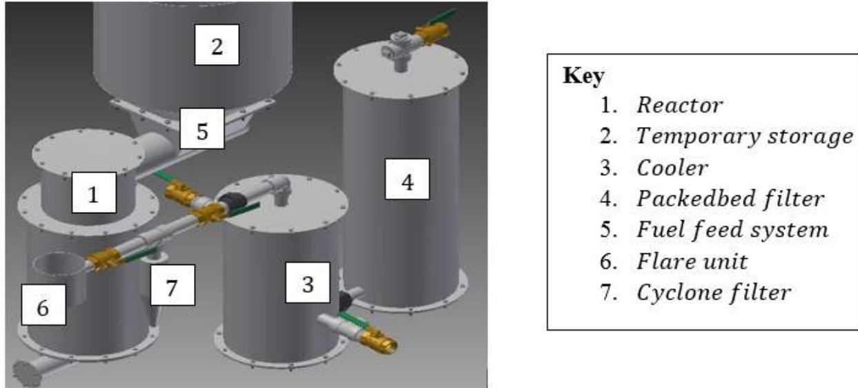
Figure 7 Starved-bed gasifier 3D solid works Design
