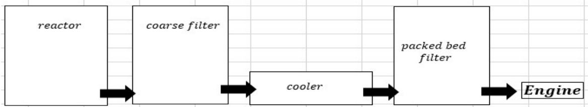
Figure 5 Prototype gasifier layout
