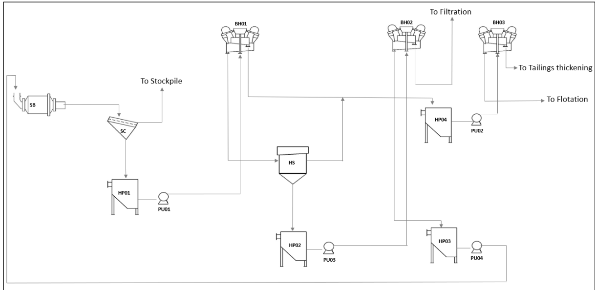
Figure 1: Simple Flowsheet of Phosphate Wash plant
