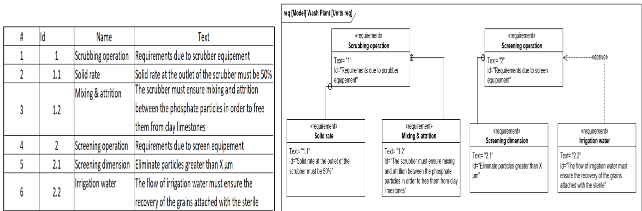
Figure 2: Different diagrams allow to capture the requirements of the Wash Plant in SysML
