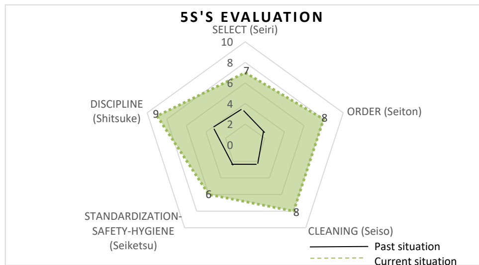
Figure 5. 5S Evaluation
