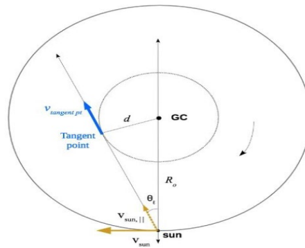
Figure 6: Relative velocity of an object to the Milky Way Source [8].
