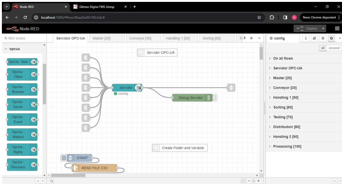
Figure 2: Node-RED Web Editor (The Authors)
