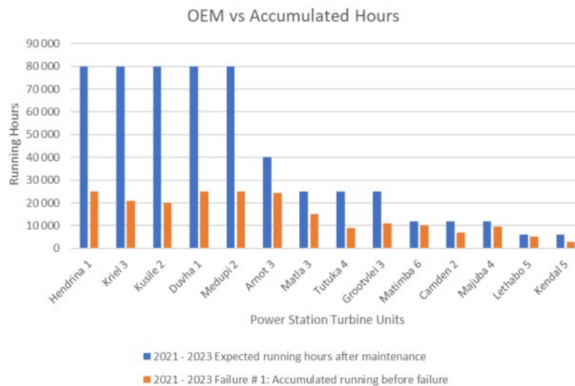
Figure 2. OEM vs Accumulated Hours Chart
