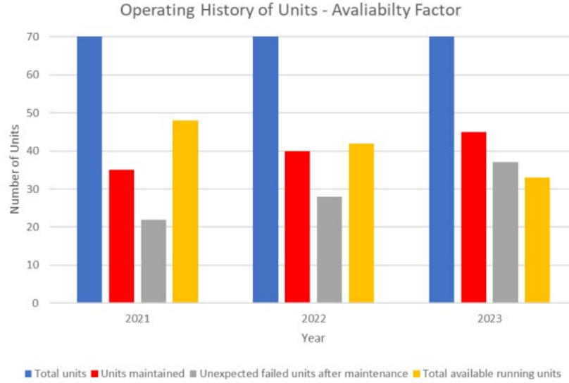
Figure 3. Steam Turbine Units Operating History Chart
