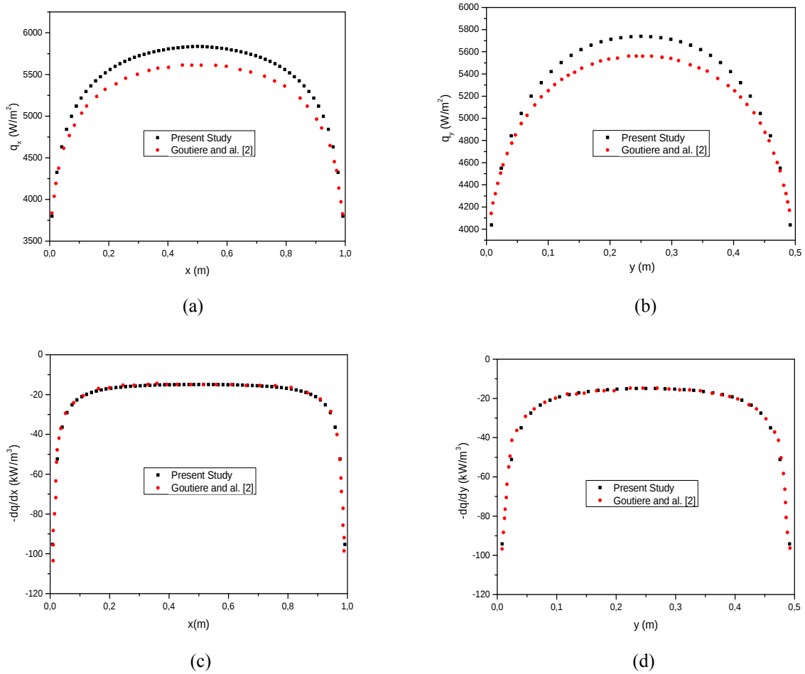
Figure 3: (a) Evolution of the heat flux q_x ; (b) Evolution of the heat flux q_y ;
