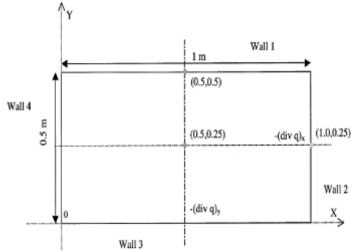
Figure 2: The enclosure
