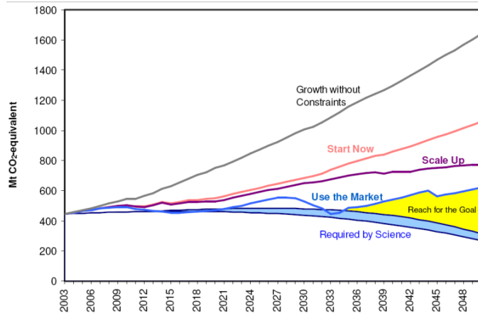
Figure 5: Carbon emission projections (Letete et al., 2009)
