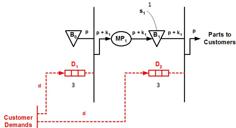
Figure 5: SS/SP/BS at t = 0
