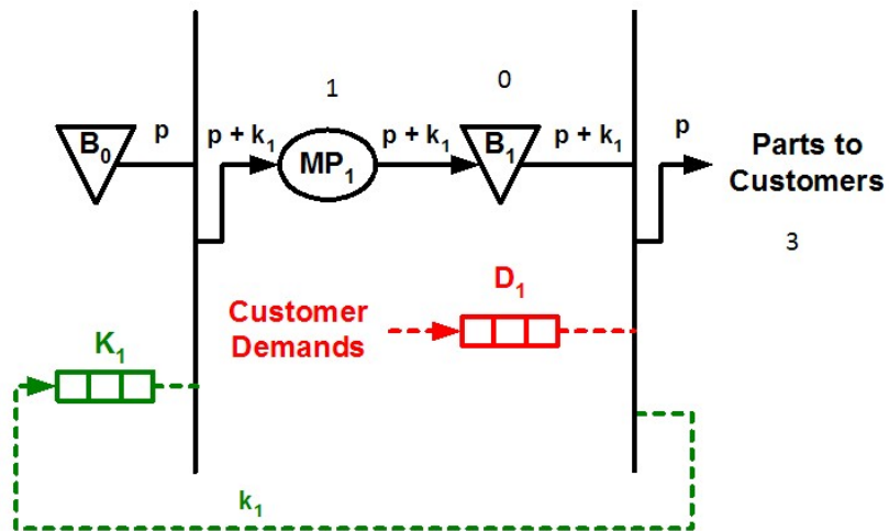
Figure 11: SS/SP/TKCS at t = 3
