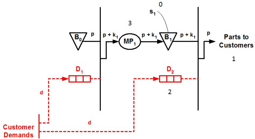
Figure 7: SS/SP/BS at t = 1
