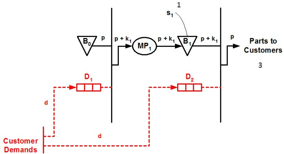
Figure 9: SS/SP/BS at t = 2
