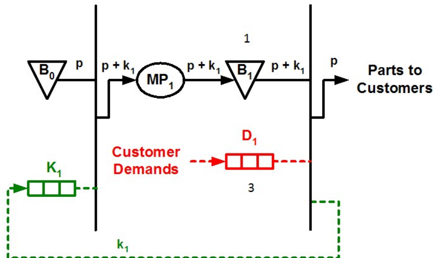
Figure 6: SS/SP/TKCS at t = 0
