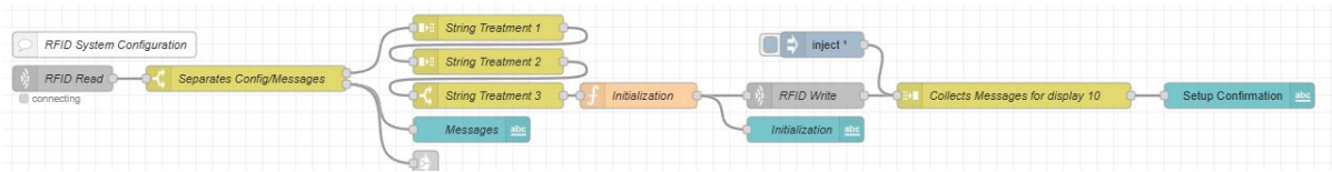
Figure 2. RFID Module Configuration (Petrocchi, 2024)
