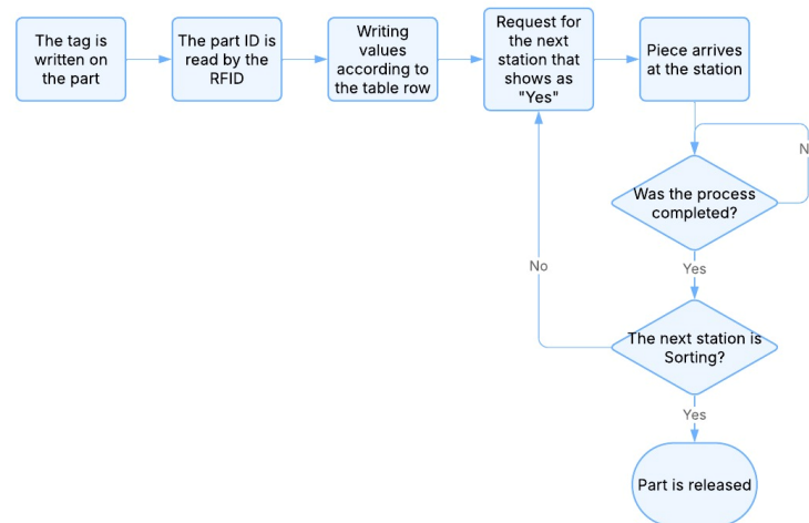
Figure 5. Proposed RFID Routing Structure
