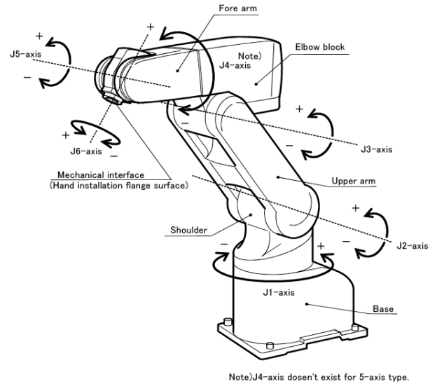
MELFA RV-2AJ Robot Arm (The authors)
