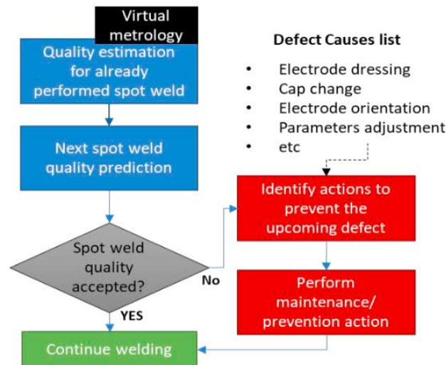
Figure 1. RSW Intelligent flow chart for zero defects (Foivos Psarommatisa 2024a)
