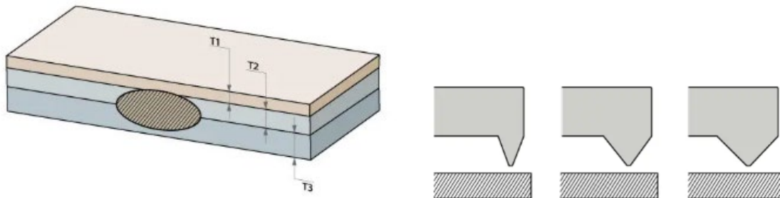
Figure 11. Spot welding Process Design
