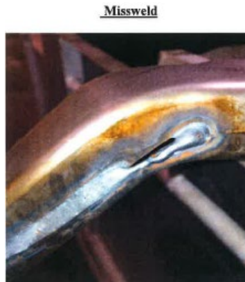
Figure 7. Missweld defects in Auto parts manufacturing
