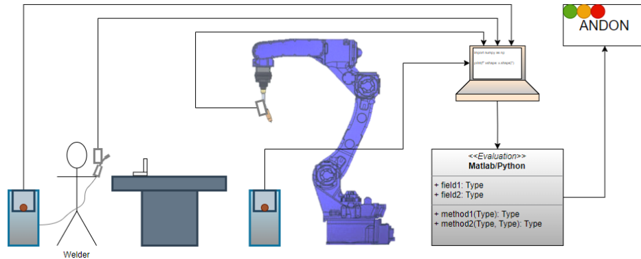
Figure 2. The RSW system with Visual Andon lights (Krist ' of Lajber 2017)
