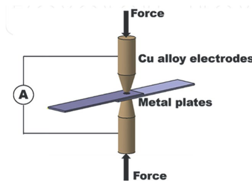
Figure 2. The schematic diagram of RSW (Tanmoy 2022)
