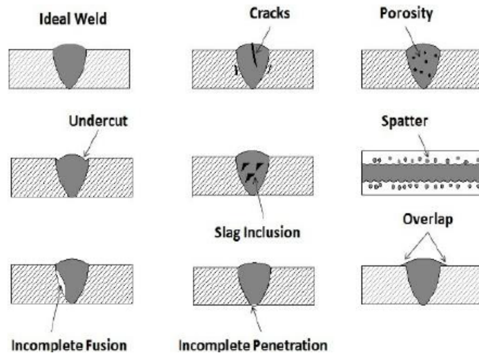
Figure 1. Welding defects (Alib 2019)
