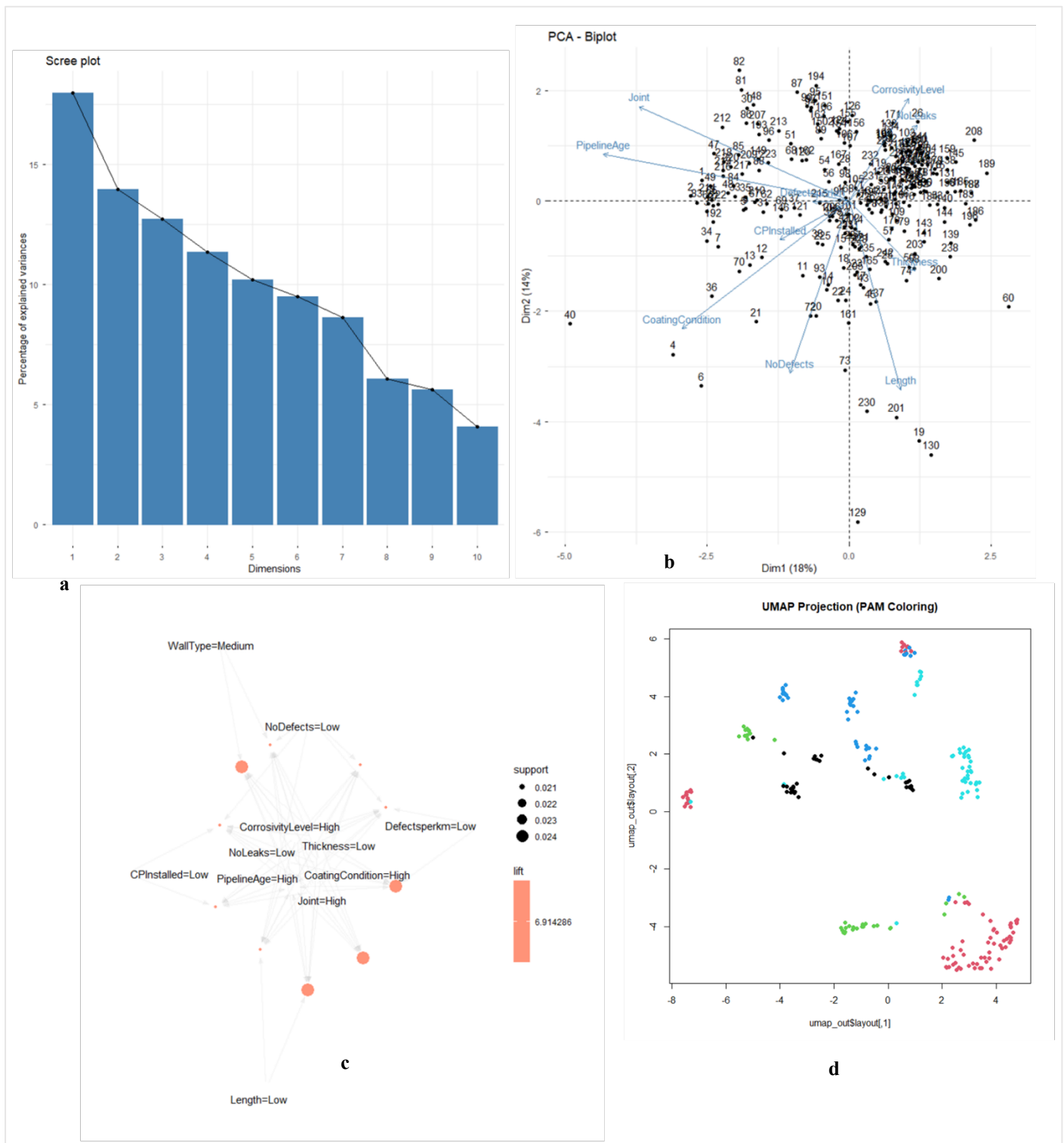
Figure 3. Dimensionality Reduction – PCA Scree Plot (a), PCA Biplot (b), Association Rule Mining (c) and UMAP (d)
