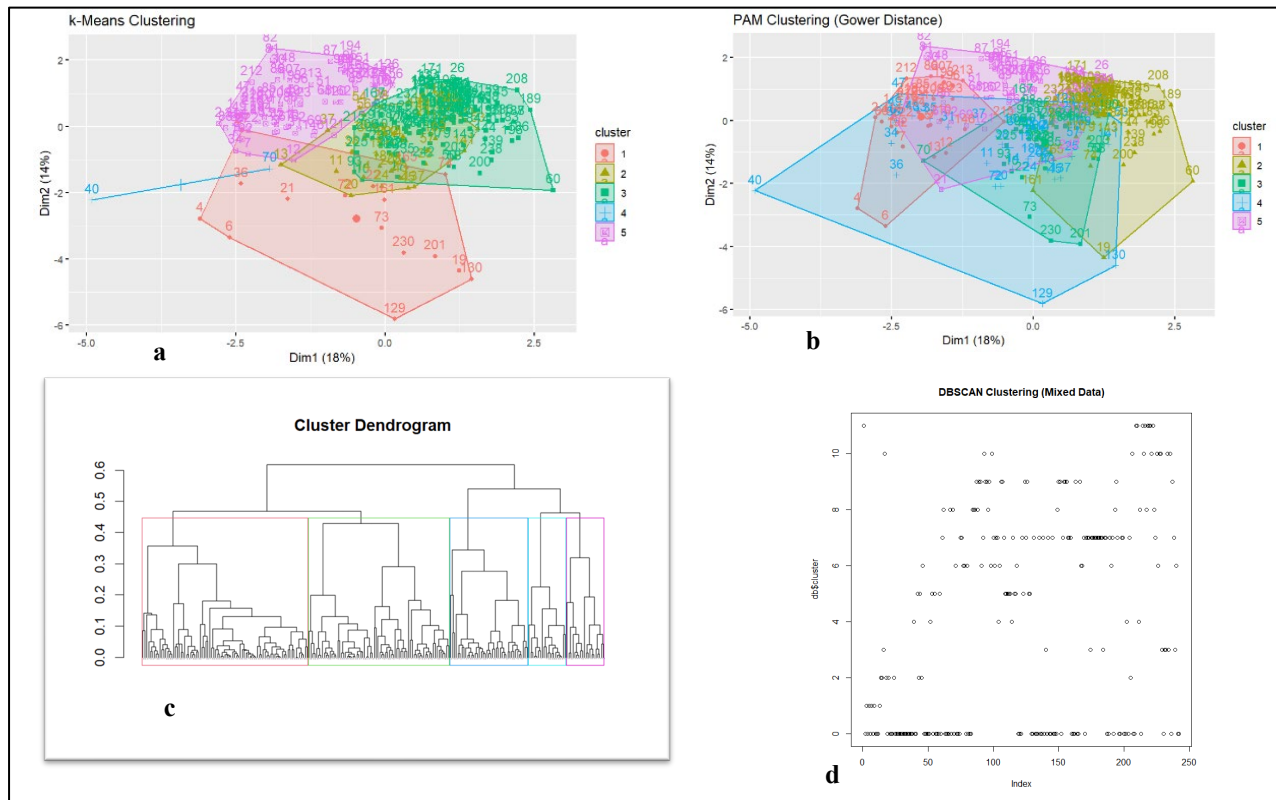
Figure 2. Clustering models-K-means Clustering (a), PAM Clustering (b), Hierarchical Clustering (c) and DBSCAN Clustering (d)
