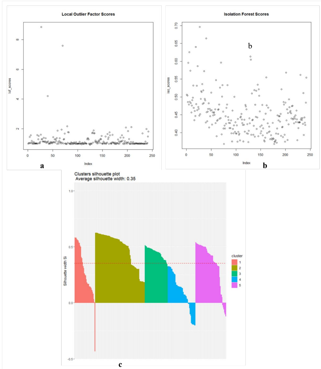
Figure 4. Cluster validation and Anomaly Detection – Local Outlier Score (a), Isolation Forest Score (b) and Silhouette (c)
