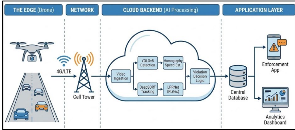
Figure 1. High-level architecture of the IATOS edge-cloud framework
